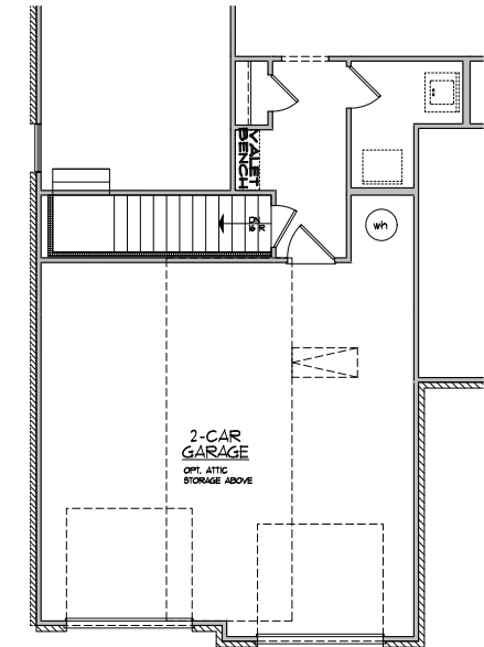
OPTIONAL BASEMENT FIRST FLOOR PLAN SCALE: 1/8"=1'-0" (11x17" SHEET SIZE)
