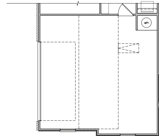
OPTIONAL 2-CAR SIDE LOAD GARAGE - ELEVATION A & C SCALE: 1/8"=1'-0" (11x17" SHEET SIZE)
