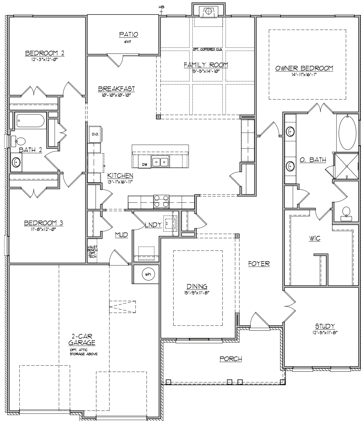
First Floor Plan - A
