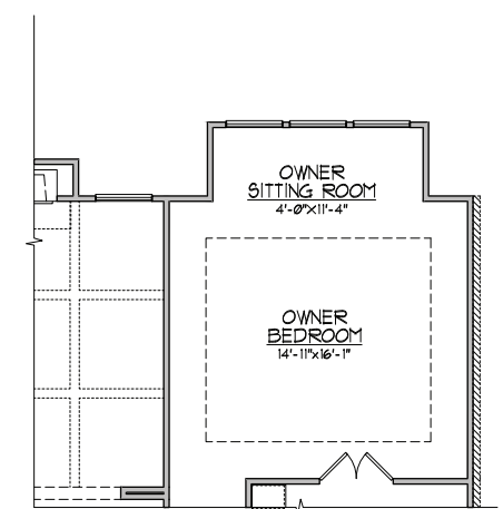
OPTIONAL OWNER SITTING SCALE: 1/8"=1'-0" (11x17" SHEET SIZE)
