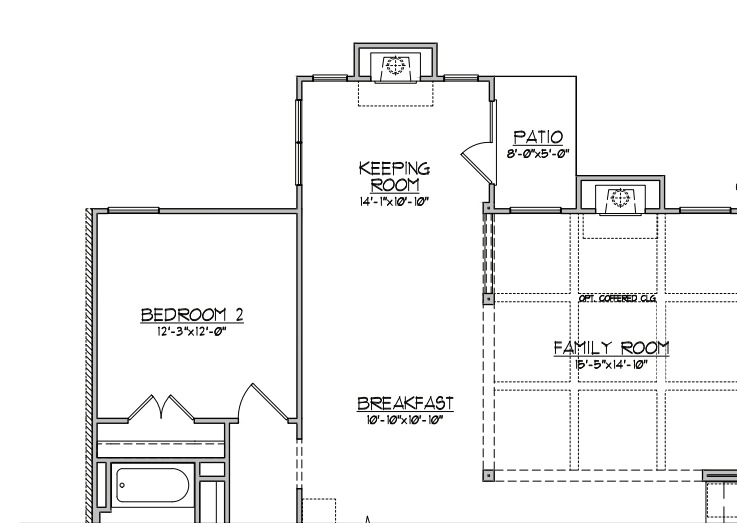
OPTIONAL KEEPING ROOM SCALE: 1/8"=1'-0" (11x17" SHEET SIZE)
