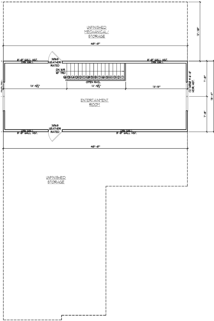
Third Floor w/Opt 5th Bedroom
