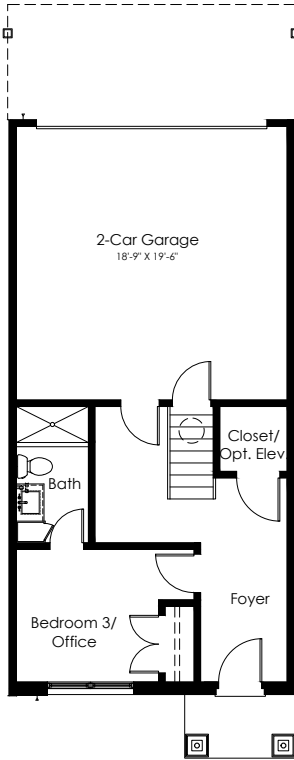
LOWER LEVEL PLAN
